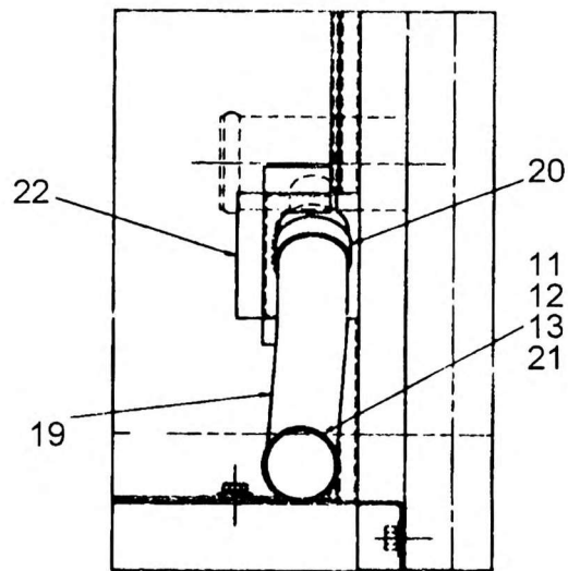
VIEW B - B
